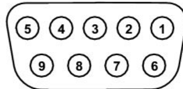
(View into Female connector)
