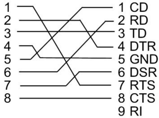
(View into Female connector)
